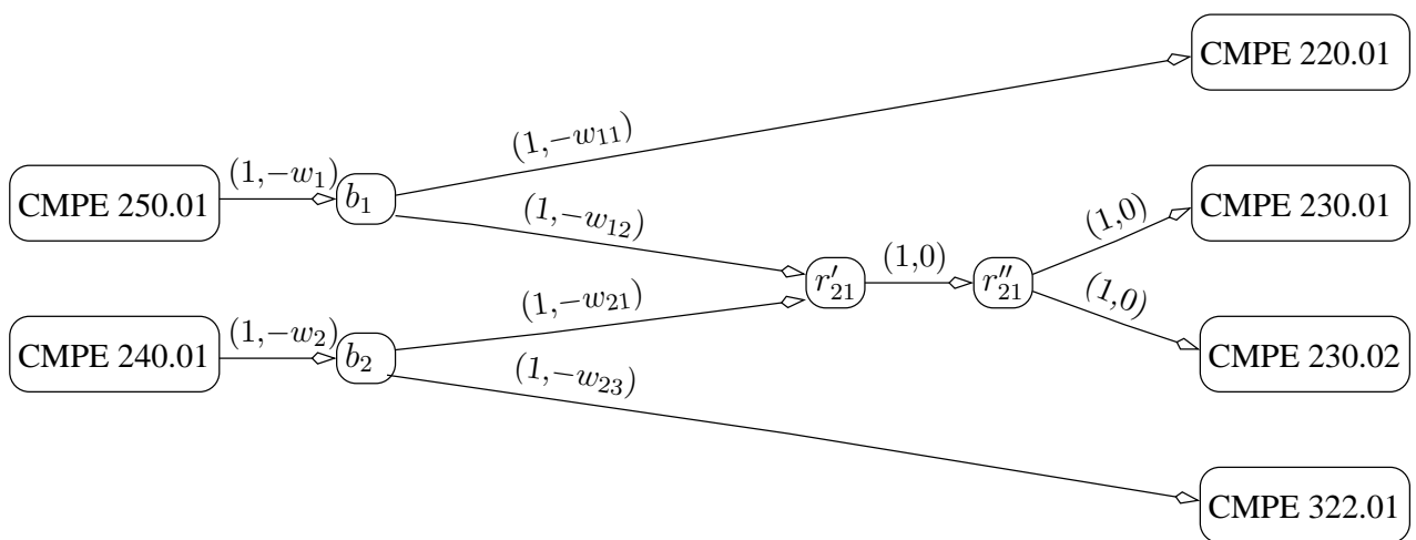
Figure 3: Network for illustrating the usage of the restriction nodes for a course restriction set with (capacity, cost) values on the arcs.
