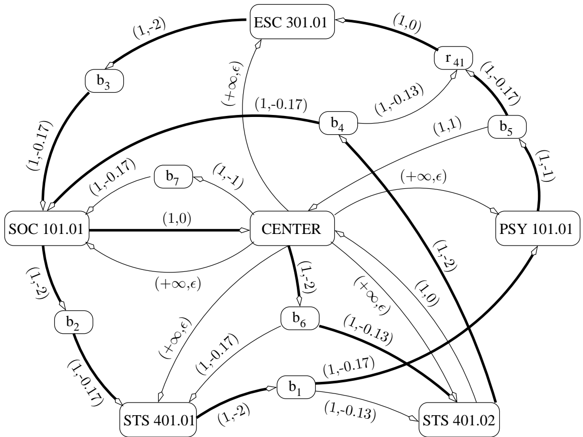
Figure 2: Minimum cost flow network of the example given in Section 2 with (capacity, cost) values on the arcs. The solution is shown with the bold arcs where one unit of flow passes in each bold arc.
