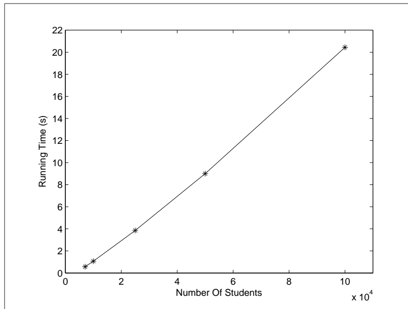
Figure 4: Graph of the number of students vs. running time (seconds) of the network solver.
