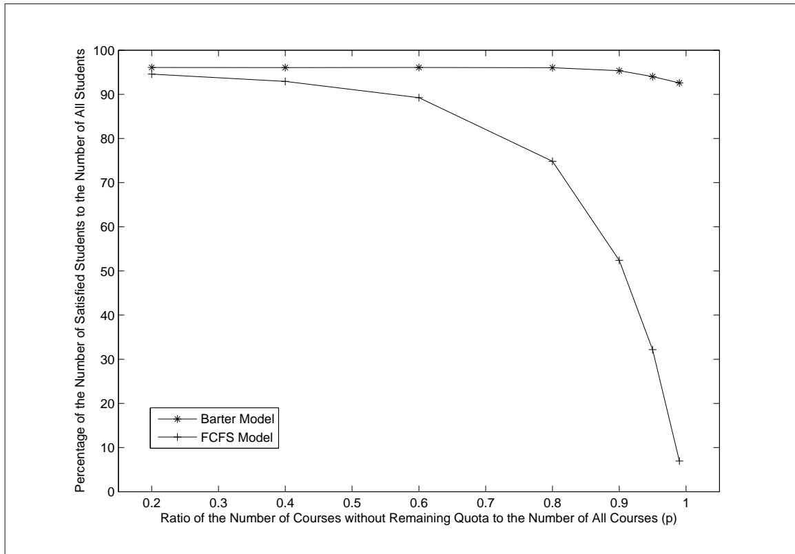
Figure 5: Graph comparing the number of satisfied students in the solutions of the barter model and the FCFS model.
